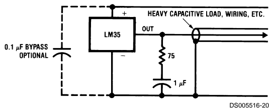
FIGURE 4. LM35 with R-C Damper
