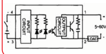
Connection Diagram
